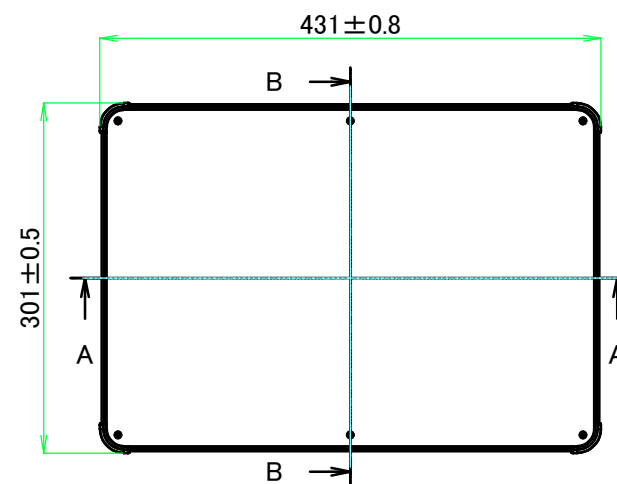
E view
